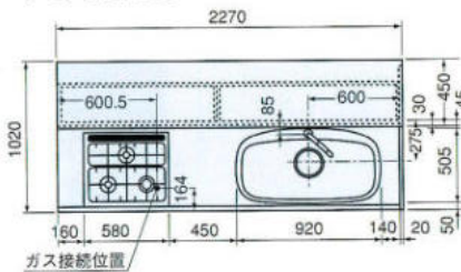
PC-225J
