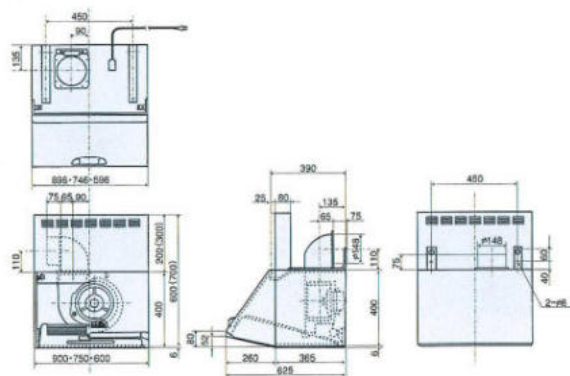
FCR-3S-602/752/902 (602H300/752H300/902H300)
