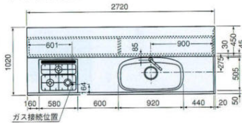
PC-270J
