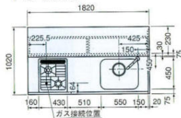
PC-180S
