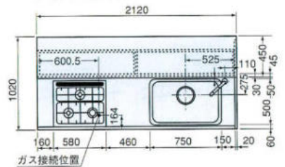
PC-210S
