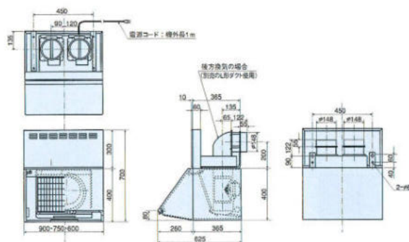
DUM-3A-601/751/901V
